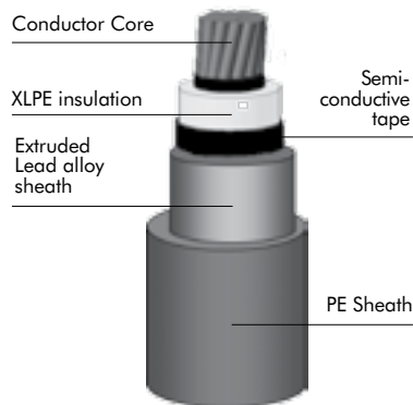
Lead Sheath
