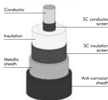
Cable components
