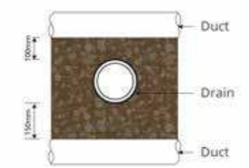
Minimum clearance between duct and drain
