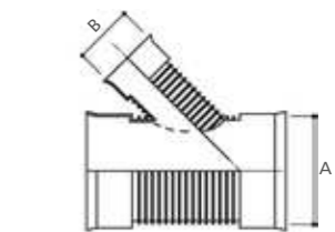
Ridgidrain 45° junctions All junctions are triple socketed. Order seals and couplings separately.
