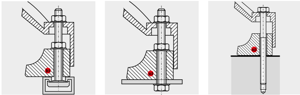
▲ Mounting types
