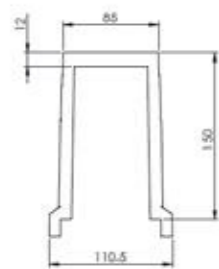
Cross Section
