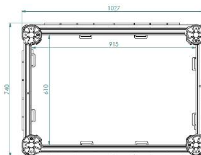
Fortress cross-section top view
