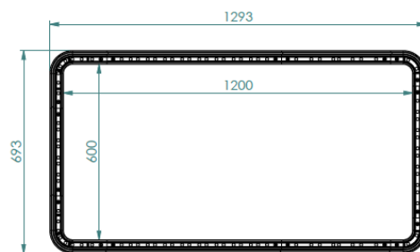
Modula cross-section top view
