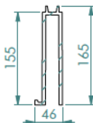
Modula cross-section detail
