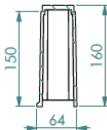
ULTIMA cross-section detail
